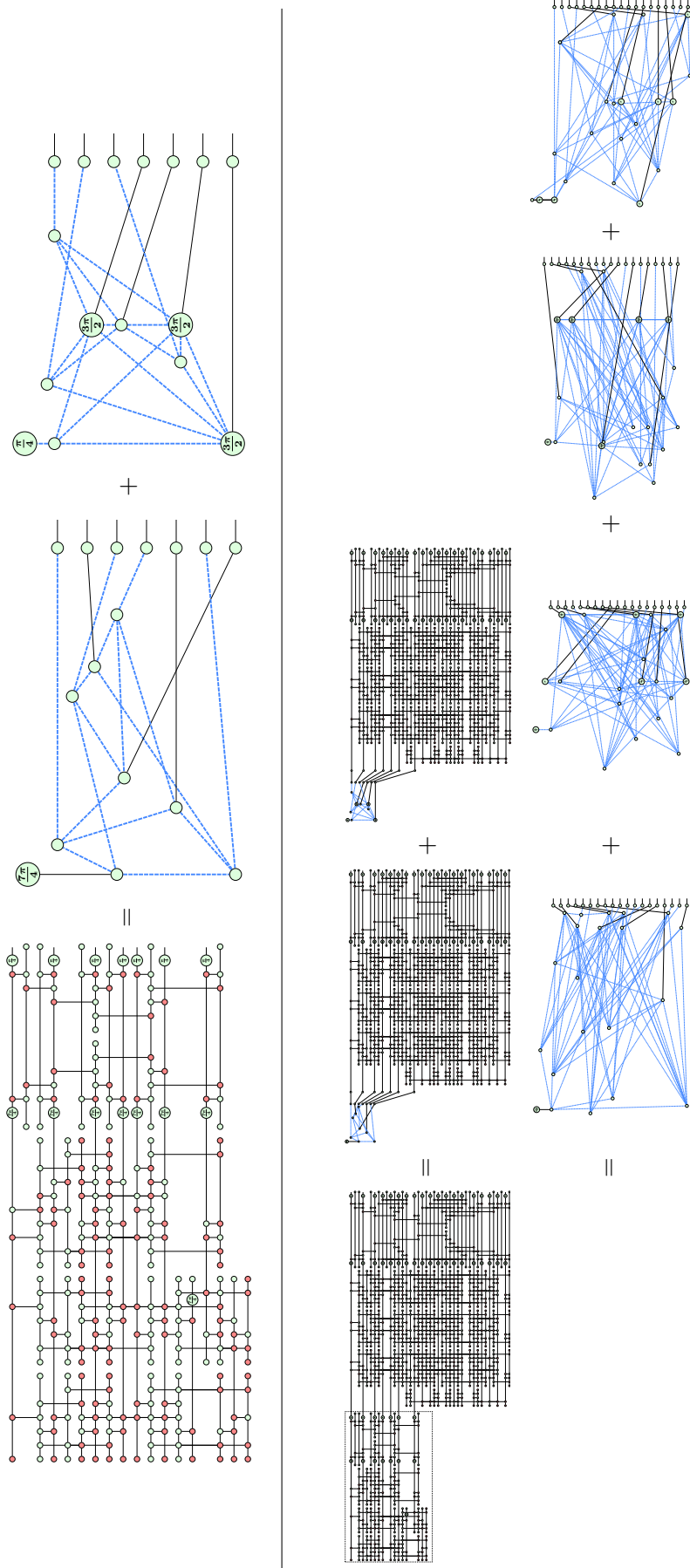
Figure 25: Cutting stabiliser decompositions of the magic state cultivation circuits. Top: the d = 3 circuit decomposes into two Clifford ZX-diagrams. Bottom: the d = 5 circuit decomposes into four Clifford ZX-diagrams via two intermediate terms.
