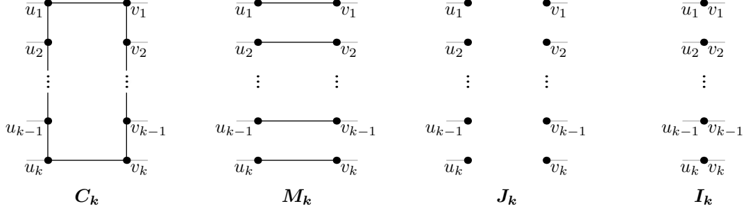
Figure 2: Atomic graphs.
