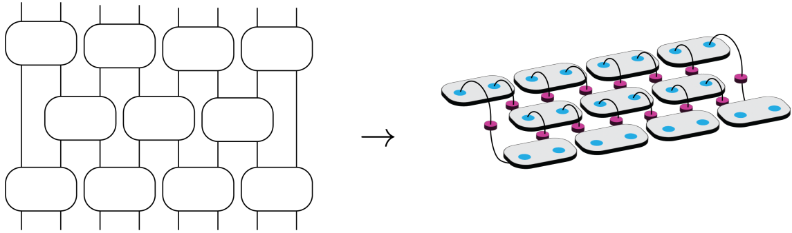
Figure 3: Graphical representation of Clifford-grid circuit parallelization. Every blue dot represents a qubit and all Clifford gates (boxes) are applied in parallel. The lines again represent Bell-state creations and Bell-state measurements, indicated by the pink boxes. The propagating Pauli errors can be corrected using the Bell-state measurement results.
