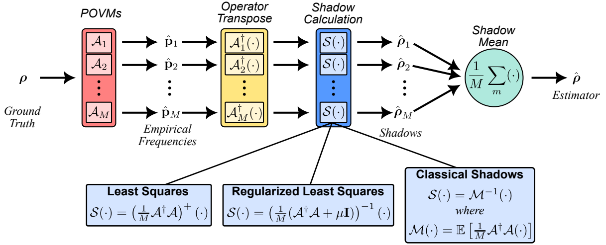
Figure 1: Shadow picture of quantum estimation. POVMs \{A_1, A_2, \dots, A_M\} \equiv \mathcal{A} are measured via repeated preparation of a ground truth quantum state \rho . The observed frequencies for each POVM produce a single shadow state \hat{\rho}_m = S(A_m^\dagger(\hat{p}_m)) , the collection of which are averaged for the final estimate \hat{\rho} . The only difference between each technique lies in the specific shadow operation chosen: (i) least squares (LS) performs the (pseudo)inverse on the POVMs directly; (ii) regularized least squares (RLS) ensures invertibility through the addition of a term proportional to the identity; and (iii) classical shadows (CS) inverts according to a simulated channel \mathcal{M} defined in expectation over all possible measurement settings.
