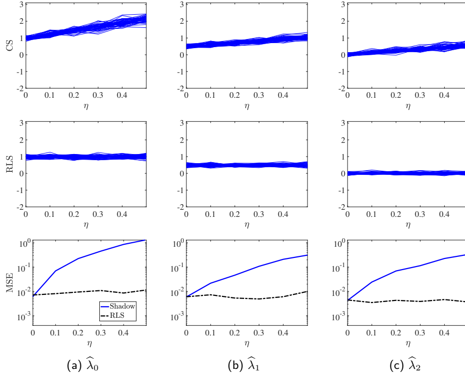
Figure 6: Illustration of the performance of the RLS and CS approaches for estimating the linear observables \lambda_i = \text{tr}(\Lambda_i \rho) in the presence of distribution shifts: the unitary matrices are generated from the distribution (1-\eta)P(\mathbb{U}_D) + \eta P((\mathbb{U}_2)^{\otimes n}) , where \mathbb{U}_D and (\mathbb{U}_2)^{\otimes n} denote the global and local Haar-distributed unitary matrices, respectively.
