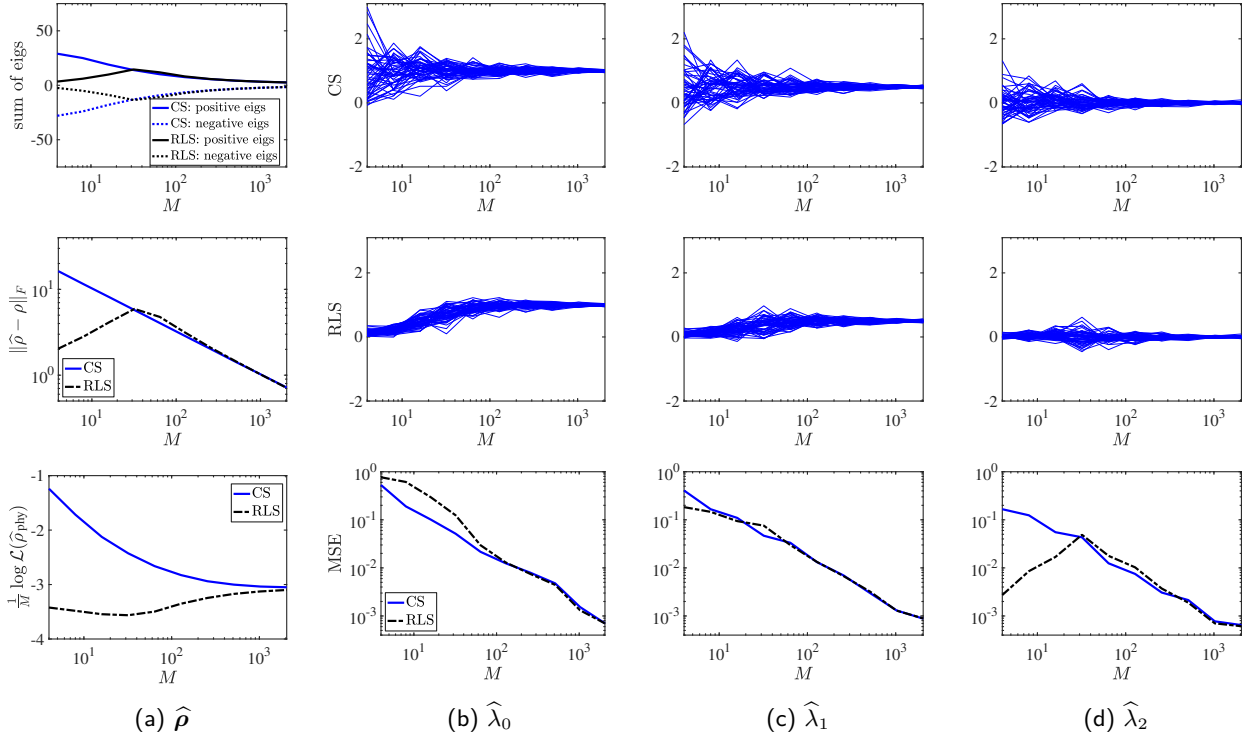
Figure 4: Illustration of the performance of CS and RLS for estimating the state \rho and the linear observables \lambda_i = \text{tr } \Lambda_i \rho with \Lambda_i = \phi_i \phi_i^\dagger .
