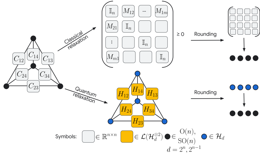
Figure 1: A cartoon description of our quantum encoding of the LNCG problem, compared to the classical formulation. (Left) The description of the problem that we consider, which is described by a graph ([m], E) and n \times n matrices C_{uv} for each edge (u, v) \in E . We wish to assign elements of \text{O}(n) or \text{SO}(n) to each vertex such that Eq. (11) is maximized. (Center top) The standard classical relaxation optimizes an mn \times mn PSD matrix M via semidefinite programming. (Right top) The classical rounding procedure, which returns a collection of orthogonal matrices from M . (Center bottom) Our quantum formulation of the problem as a two-body fermionic Hamiltonian. On each vertex we place a d -dimensional Hilbert space, with interaction terms H_{uv} on the edges constructed from each C_{uv} . The classical solution to the LNCG problem lies as a subset of this full Hilbert space. (Right bottom) Our proposed quantum rounding protocols. One protocol requires knowledge of the two-body reduced density matrices across edges, while the other uses the one-body reduced density matrices on each vertex.
