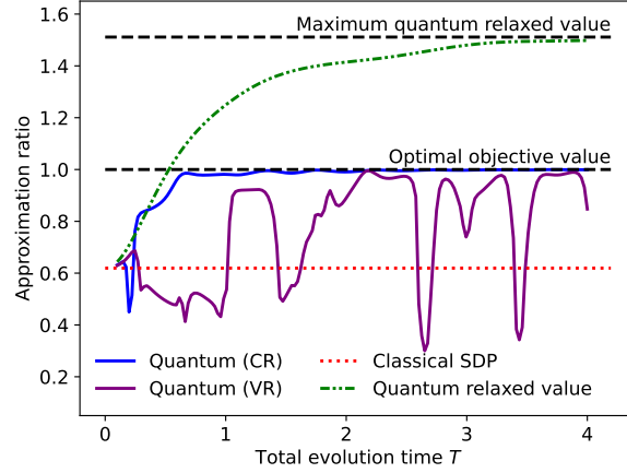
Figure 3: Demonstration of a typical instance of adiabatic state preparation for preparing relaxed quantum solutions. The initial state is the product of Gaussian states corresponding to the rounded solution of the classical SDP. As the total evolution time T increases, the evolution becomes more adiabatic, indicated by the convergence of the relaxed value to the maximum eigenvalue (in units of the original problem's optimal value). The rounded solutions of course can never exceed the original problem's optimal value.
