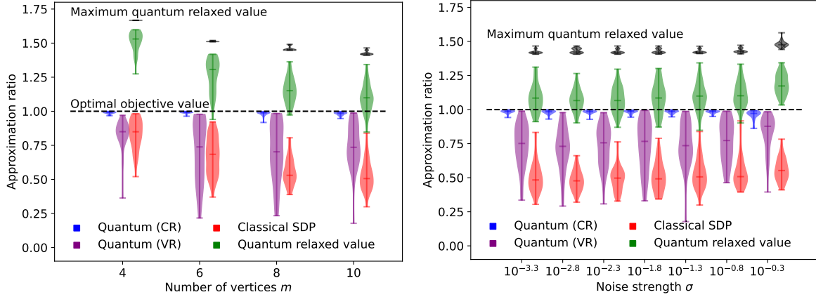
Figure 4: Approximation ratios for solutions obtained from rounding the “adiabatically” evolved state |\psi(T)\rangle with fixed T = 1 for all m, \sigma . Problem instances and visualization is the same as in Figure 2. We also include the maximum eigenvalue of the relaxed Hamiltonian and the energy of the prepared unrounded state, to demonstrate how far |\psi(T)\rangle is from the exact maximum eigenvector. (Left) Varying the number of vertices m in the graph. Note that the number of qubits required here is 2m . (Right) Varying the noise strength parameter \sigma .
