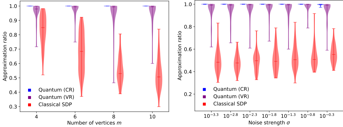
Figure 2: Approximation ratios for solutions obtained from rounding the maximum eigenvector of the relaxed Hamiltonian \tilde{H} . Violin plots show the distribution of approximation ratios over 50 randomly generated instance, and with the median being indicated by the center marker. CR refers to rounding according to the conv \text{SO}(n) -based scheme (Section 7.3), while VR denotes the vertex-marginal rounding scheme (Section 7.4). The classical SDP solution was rounded by the standard randomized algorithm [16], and we report the best solution over 1000 rounding trials. (Left) Varying the number of vertices m in the graph (random 3-regular graphs). Note that the number of qubits required here is 2m . (Right) Varying the noise strength parameter \sigma which defines the problem via C_{uv} = g_u g_v^\top + \sigma W_{uv} .
