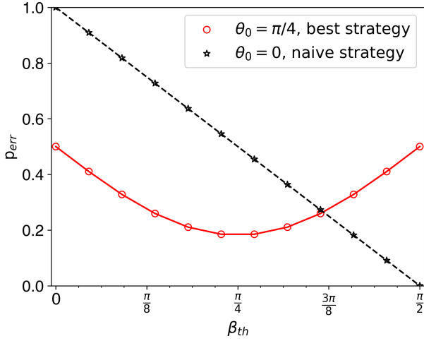
Figure 5: The probability of making wrong decision versus the decision threshold \beta_{\text{th}} . Data shown for a binary decision of displacement sensing using degree-1 bosonic QSP with \kappa = 1 , comparing the best ( \theta_0 = \pi/4 , red circle) and the naïve ( \theta_0 = 0 , black star) sensing protocol.
