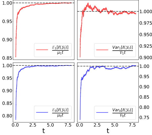
Figure 4: Damping-rate discrimination . We show the ratio between theoretical and numerically-computed values of the mean value (variance) in the first (second) column, as a function of time, when sampling from hypothesis h_{1(0)} in the first (second) row; these results were computed over 2 \cdot 10^4 quantum trajectories. As observed, after a transient time, the first and second moments converge to the predicted analytical values.
