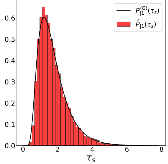
Figure 7: Damping-rate discrimination . We compute the histogram of the stopping times for the sequential test and compare it with the Inverse Gaussian probability distribution of theorem 4, showing a good agreement. Results are shown when h_1 holds true (similar results are obtained when swapping the underlying hypothesis).
