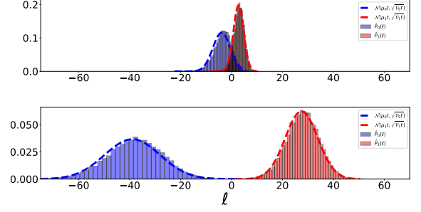
Figure 5: Damping discrimination . We show the histogram of the LLR for time t = 2s ( t = 8s ) in the upper (lower) panel, under hypothesis h_{1(0)} in red (blue). We compare this with the theoretically predicted Gaussian distributions
