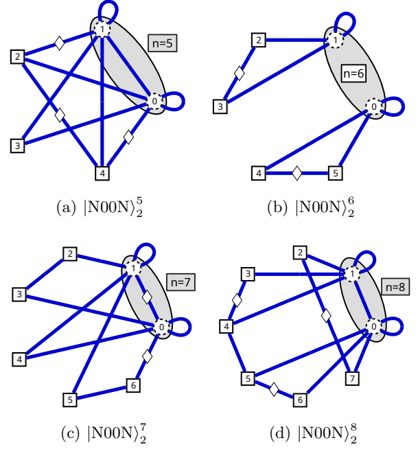
Figure 38: Graphs for two-mode N00N states of 5, 6, 7, and 8 photons.
