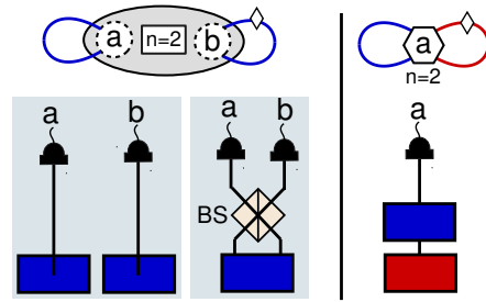
Figure 6: Graphs for producing |N00N\rangle_2^2 states and the related experiments. On the left side, the graph with two blue edges (i.e., two self-loops) is for a path-entangled N00N state (|2, 0\rangle_{a,b} - |0, 2\rangle_{a,b})/\sqrt{2} . We translate this graph into several setups (below the graph). The setups using path identity or path encoding are the same in this case. With bulk optics, one can achieve the state with a Hong-Ou-Mandel interferometry [87, 20], where two identical photons enter a 50:50 beam splitter. One can also perform such a state in polarization, i.e., (|2, 0\rangle_{H,V} - |0, 2\rangle_{V,H})/\sqrt{2} on the right side. The blue and red colors are, respectively, for horizontal and vertical polarization. The coherent superposition of blue and red self-loops gives the N00N state. Its related setup is described below the graph. There either two horizontally polarized photons (blue edge) or two vertically polarized photons (red edge) are in path a with a single-photon sensitive detector.
