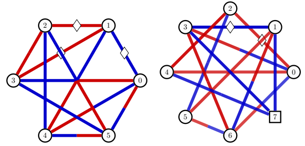
Figure 31: k=2 uniform state for 6 qubits and k=2 (almost) uniform state for 7 qubits (+ one ancilla).
