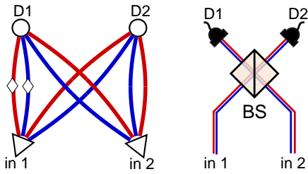
Figure 9: An abstract graph for Bell state measurement. A measurement event happens if the photons in1 and in2 are in the Bell state |\Psi^-\rangle . Simultaneous clicks in the detectors D1 and D2 signify a successful Bell measurement. The corresponding setup is given for the graph, which is a typical Bell state measurement setup.
