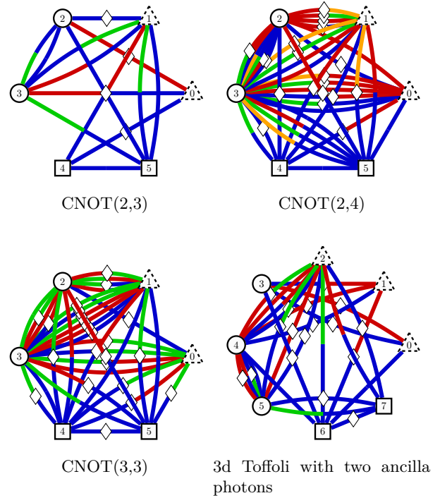
Figure 60: Graphs for quantum gates with post-selection.
