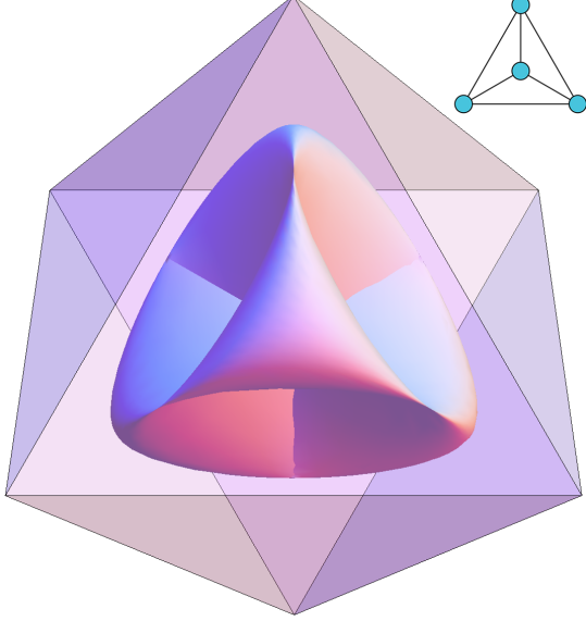
Figure 1: The three-fold degeneracy region D_{\mathbb{R}} of the tetrahedron graph inside the octahedronal density domain. The corners of the octahedron correspond to the extreme density (1, 1, 0, 0) and its permutations, generalized barycentric coordinates are used to display densities.
