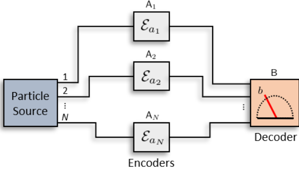
Figure 1: A physical implementation of the MAC p_{B|A} using a single particle and a generalized interferometer setup.
