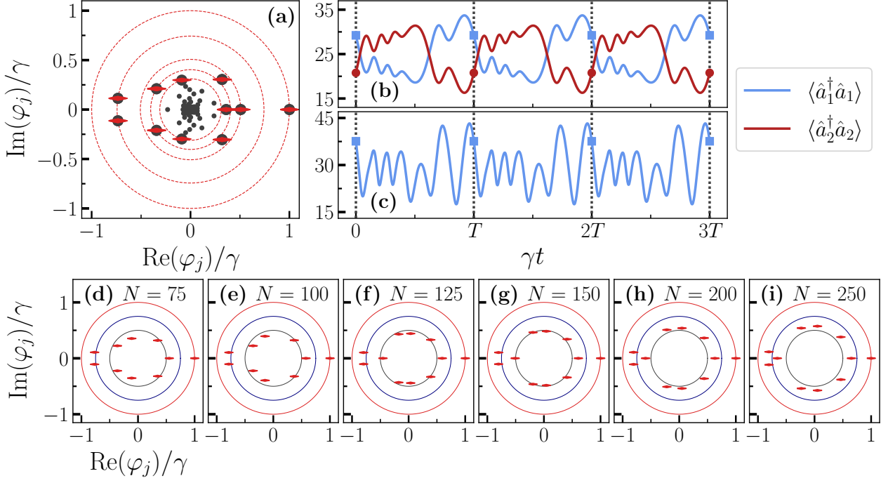
Figure 8: Results for the Bose-Hubbard dimer with a time dependent modulation presented in Eq. (36) and dissipation presented in Eq. (37). The chosen parameters, i.e., UN/J = 1 , f_0/J = 1 , f_1/J = 3.4 , \omega/J = 1 , and \gamma N/J = 0.2 , match those from Ref. [85] (to be consistent with our notation, a multiplication with a factor 2 was applied to \gamma ). (a), (b), and (c) are for N = 50 . (a) Spectrum of the Floquet map \mathcal{F} obtained via exact diagonalization (gray dots) and our method for the 10 slowest states and their complex conjugates (red horizontal markers). The dashed lines represent the circles with radius equal to the absolute value of the eigenvalue \varphi_j . (b) The particle number expectation value \langle \hat{a}_1^\dagger \hat{a}_1 \rangle and \langle \hat{a}_2^\dagger \hat{a}_2 \rangle , time evolved from the stroboscopic steady state \hat{\rho}_{\text{ss}}^F \propto \hat{\rho}_0^F obtained with our algorithm, i.e., the state whose eigenvalue is \varphi_0 = 1 . (c) As a function of time, the real part of the particle number expectation value of the first cavity \langle \hat{a}_1^\dagger \hat{a}_1 \rangle (coinciding with that of the second cavity) for the slowest decaying state \hat{\rho}_1^F obtained with our algorithm, rescaled by the exponential damping \exp(|\varphi_1|t) . Given the degeneracy in the real part of \varphi_1 and \varphi_2 , we assigned the value \varphi_1 to the one with negative imaginary part. Panels (d)–(i) the 10 largest eigenvalues (and their complex conjugates) of \mathcal{F} (red horizontal markers) are shown for (d) N = 75 , (e) N = 100 , (f) N = 125 , (g) N = 150 , (h) N = 200 , and (i) N = 250 . The red circle depicts the unit circle, the blue circle is the circle with radius 0.75, and the gray circle has radius 0.5.
