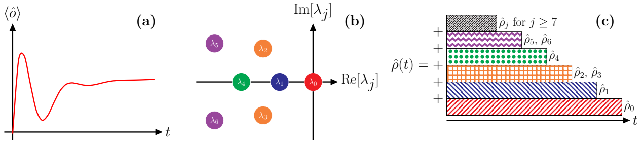
Figure 1: Pictorial representation of the physical meaning of the time evolution of a density matrix from a spectral point of view. (a) The dynamics of a system governed by a Lindblad master equation has always some common characteristics. Indeed, after an initial transient dynamics, the system converges to its steady state. (b) These characteristics are clear from a Liouvillian spectrum point of view. Except from the steady state \hat{\rho}_0 characterized by \lambda_0 = 0 , the eigenvalues characterizing the Liouvillian eigenmatrices have always non-positive real part (they describe decaying processes towards the steady-state) and they always appear as complex conjugate (they preserve the Hermiticity of a density matrix). (c) This translates in a specific form of the density matrix along its evolution. While at the beginning all the eigenmatrices are relevant, as time passes the coefficients of the eigenmatrices \hat{\rho}_j whose eigenvalues \lambda_j have large negative part become negligible. But while at long time \hat{\rho}_j with large j are irrelevant, the slow-decaying eigenmatrices (including the steady state) are present also in the short-time dynamics. Thus, by just doing long-time evolution, we are discarding all the possible information on \hat{\rho}_j derived from the short-time dynamics.
