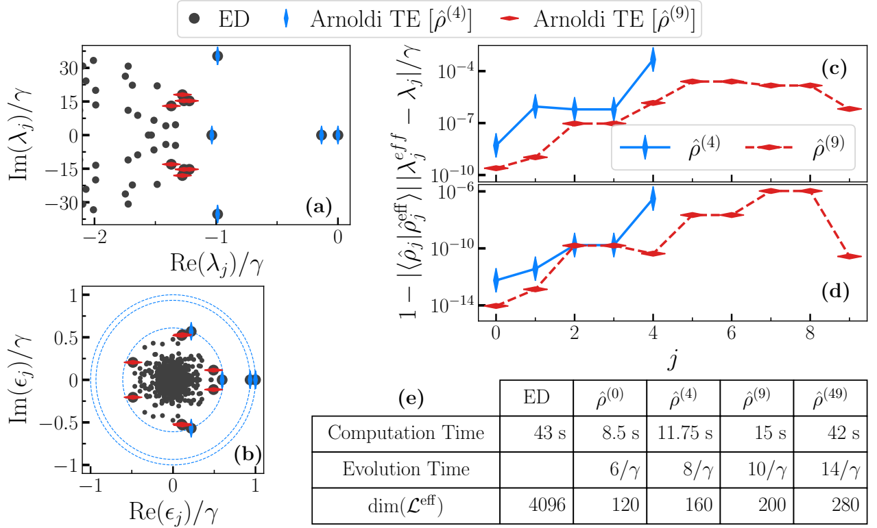
Figure 3: Bose Hubbard dimer for the parameters \Delta = 5\gamma , F_1 = F_2 = 4.5\gamma , U = 20\gamma , and J = 10\gamma , a cutoff n_{max} = 7 and T = \gamma/20 . The results are for: Exact diagonalization (ED, gray dots); our method, the Arnoldi-Lindblad time evolution for the 5 slowest states \hat{\rho}^{(4)} (blue curves and vertical markers) and for the 10 slowest states \hat{\rho}^{(9)} (red curves and horizontal markers). (a) Comparison of the Liouvillian spectrum obtained via ED and our method. (b) Spectrum of the evolution operator obtained via ED and our method. The dashed lines represent the circles whose radius is the absolute value of \epsilon_j (c.f. Fig. 2). For the sake of graphical clarity, in this panel we considered T = \gamma/2 in order to make the eigenvalues more distant. (c) Difference between the eigenvalues obtained with the ED \lambda_j and our method \lambda_j^{\text{eff}} for \hat{\rho}^{(4)} and \hat{\rho}^{(9)} . (d) One minus the absolute value of the overlap between the eigenmatrices obtained via the ED and our method for \hat{\rho}^{(4)} and \hat{\rho}^{(9)} . (e) Overview of the computational effort required for each task on our local machine [Intel(R) Xeon(R) W-2135 CPU @ 3.70GHz (12 CPUs) and 128 Gb of RAM].
