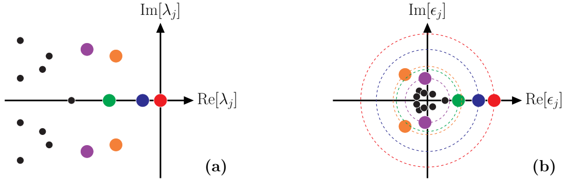
Figure 2: Spectrum of the Liouvillian [dots in (a)] vs spectrum of the corresponding evolution operator [dots in (b) with the same color]. While the steady state is the zero of the Liouvillian (red dot), \epsilon_0 is the largest eigenvalue of \mathcal{E} , as it can be seen in (b), where the dashed lines represent the circles of radius |\epsilon_j| = \exp[\text{Re}(\lambda_j)] . Thus, the Arnoldi iteration is well suited to obtain \hat{\rho}_0 from \mathcal{E} . Furthermore, the eigenvalues with the smallest real part acquire the larger magnitude [other colored dots in (a) and (b)], while the fast-decaying processes are condensed towards the zero (black dots).
