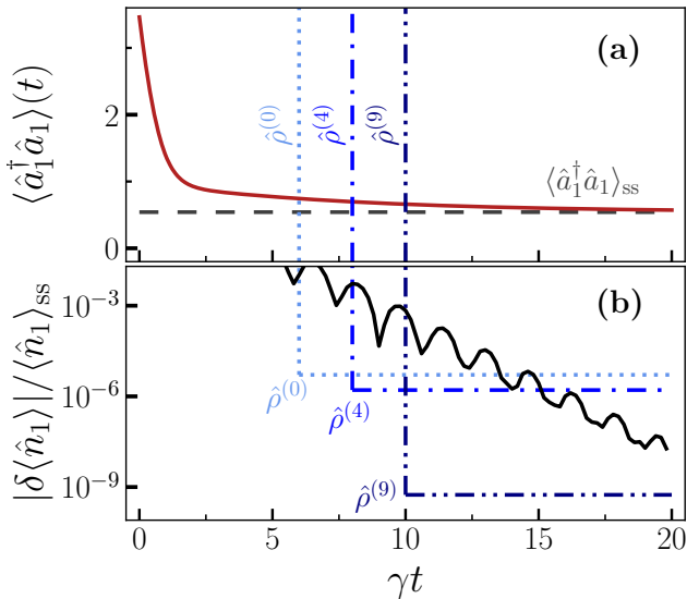
Figure 4: (a) Time evolution of the expectation value of the particle number of the first cavity of the dimer \hat{n}_1 = \langle \hat{a}_1^\dagger \hat{a}_1 \rangle (red full line). The steady-state solution obtained via exact diagonalization, i.e. \langle \hat{a}_1^\dagger \hat{a}_1 \rangle_{ss} (gray horizontal dashed line). The time when our method reaches convergence for \hat{\rho}^{(m)} is shown by vertical lines for m = 0 (light-blue dotted line), m = 4 (blue dash-dotted line) and m = 9 (dark-blue dashed-dotted-dotted line). (b) Relative difference between the expectation value \langle \hat{n}_1 \rangle obtained via ED and either our method or a fit of the exponential decrease towards the steady state (black solid line). The fit of \langle \hat{n}_1 \rangle_{ss} via Eq. (22) has been done with the curve_fit function of the SciPy library [110], and the curve plotted here is a rolling average over a time 0.08\Gamma . Same parameters and initial state as in Fig. 3.
