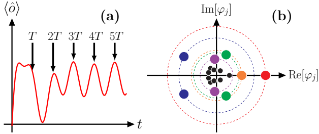
Figure 7: Time evolution of a time-dependent and periodic Liouvillian superoperator. (a) As in Fig. 1(a), but for a Liouvillian of period T . By monitoring the system every period T , the system converges to a stroboscopic stationary regime after an initial transient dynamics. (b) By introducing the Floquet map \mathcal{F} , these characteristics are clear. Except from the stroboscopic steady state \hat{\rho}_0 characterized by \varphi_0 = 1 , the eigenvalues characterizing the Floquet map eigenmatrices lie inside the unit circle, indicating decaying processes. Notice also the similarity between the spectrum of \mathcal{F} and that of the evolution operator of a time-independent Lindblad master equation \mathcal{E} in Fig. 2.
