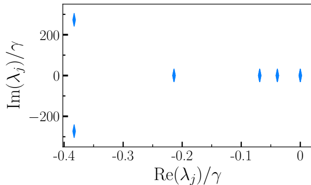
Figure 5: Results for \hat{\rho}^{(5)} of the Bose Hubbard trimer for the parameters \Delta = 5\gamma , F_1 = F_2 = 4.5\gamma , U = 20\gamma , and J = 10\gamma . This is the same set of parameters as in Fig. 3, having opportunely rescaled J by the connectivity z . The results were obtained for the convergent cutoff n_{max} = 7 . These results were obtained after a computation time of less than 1 hour on our local machine.
