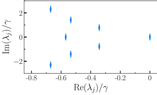
Figure 6: Results of \hat{\rho}^{(8)} for a Bose-Hubbard dimer with asymmetrical drive. The parameters are F_1/\gamma = 8 , F_2 = 0 , U/\gamma = 1/8 , \Delta/\gamma = 2 , and J/\gamma = 2 as in Ref. [62]. The local Hilbert space has a cutoff at n_{\max} = 27 . We obtained these results with a simulation of less than two hours.
