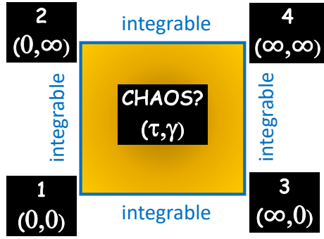
Figure 1: Depiction of the (compactified) (\tau, \gamma) parameter space window \tau \in [0, \infty) and \gamma \in [0, \infty) . At the four corners of the window, the Hamiltonian H(N, W, \tau, \gamma) has exact solutions and is superintegrable. The four edges connecting these corners are integrable models where exact solutions can be found by the solution of coupled transcendental equations. Except for possibly the case of N = 2 , the H(N, W, \tau, \gamma) does not appear integrable or solvable for arbitrary (\tau, \gamma) in this parameter space
