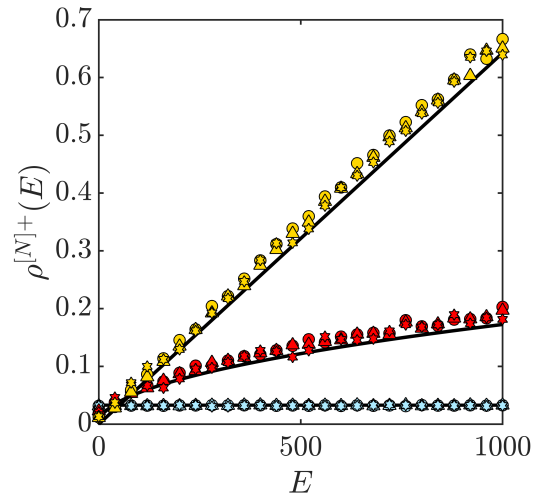
Figure 2: Density of states for N = 2 (blue points), N = 3 (red points) and N = 4 (yellow points). Solid lines show the leading term in Eq. (2) for the respective particle numbers. Symbols denote different system parameters: \gamma = 10 and \tau = 0 (circles), \gamma = \tau = 10 and W = 2 (triangles) and \gamma = \tau = 10 and W = 10 (stars).
