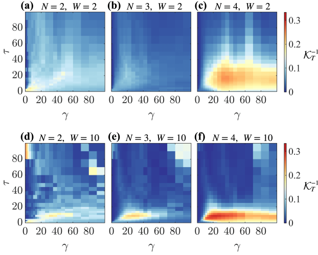
Figure 5: Inverse of the kurtosis \mathcal{K}_T^{-1} as a function of \tau and \gamma for (a,d) N = 2 (b,e) N = 3 and (c,f) N = 4 particles. The number of wells are (a-c) W = 2 and (d-f) W = 10 . For W = 2 the minimum kurtosis is 4.3592 at \gamma = 30 and \tau = 15 , while for W = 10 the minimum kurtosis is 3.3274 at \gamma = 20 and \tau = 7.5 .
