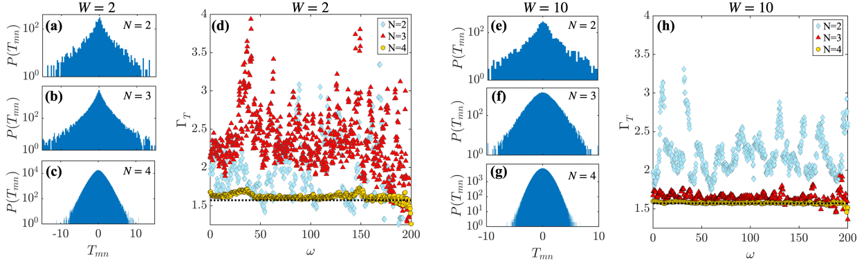
Figure 6: Off-diagonal elements of the kinetic energy operator T_{mn} for (a-d) W = 2 wells and (e-h) W = 10 wells. The probability distributions in the respective potentials are shown for (a,e) N = 2 (b,f) N = 3 and (c,g) N = 4 . (d,h) The ratio \Gamma_T as a function of \omega = |E_m - E_n| in an energy window at E_{\text{mid}} = 700 and width \Delta E = 100 . The interaction strengths and barrier heights are chosen at the point of minimum kurtosis for 4 particles in Fig.5(c,f), namely \gamma = 30 and \tau = 15 for W = 2 , and \gamma = 20 and \tau = 7.5 for W = 10 .
