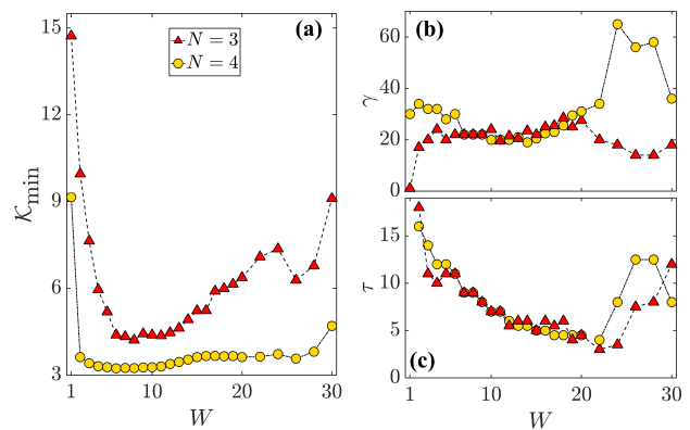
Figure 8: (a) Minimum of the kurtosis as a function of the number of wells for N = 3 (red triangles) and N = 4 (yellow circles). Kurtosis is calculated in an energy window of width \Delta E = 100 around E_{\text{mid}} = 700 . (b) Interaction and (c) barrier height corresponding to the points of minimum kurtosis in (a).
