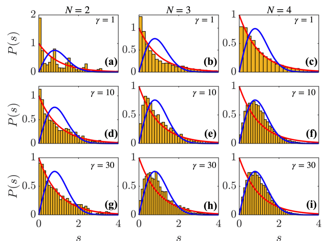
Figure 3: Energy level spacing distributions for (a,d,g) N = 2 particles, (b,e,h) N = 3 particles and (c,f,i) N = 4 particles with different interaction strengths \gamma . The barrier height is fixed to \tau = 10 and the number of wells is W = 2 . The red solid line is the Poissonian distribution and the blue solid line is the Wigner-Dyson distribution.
