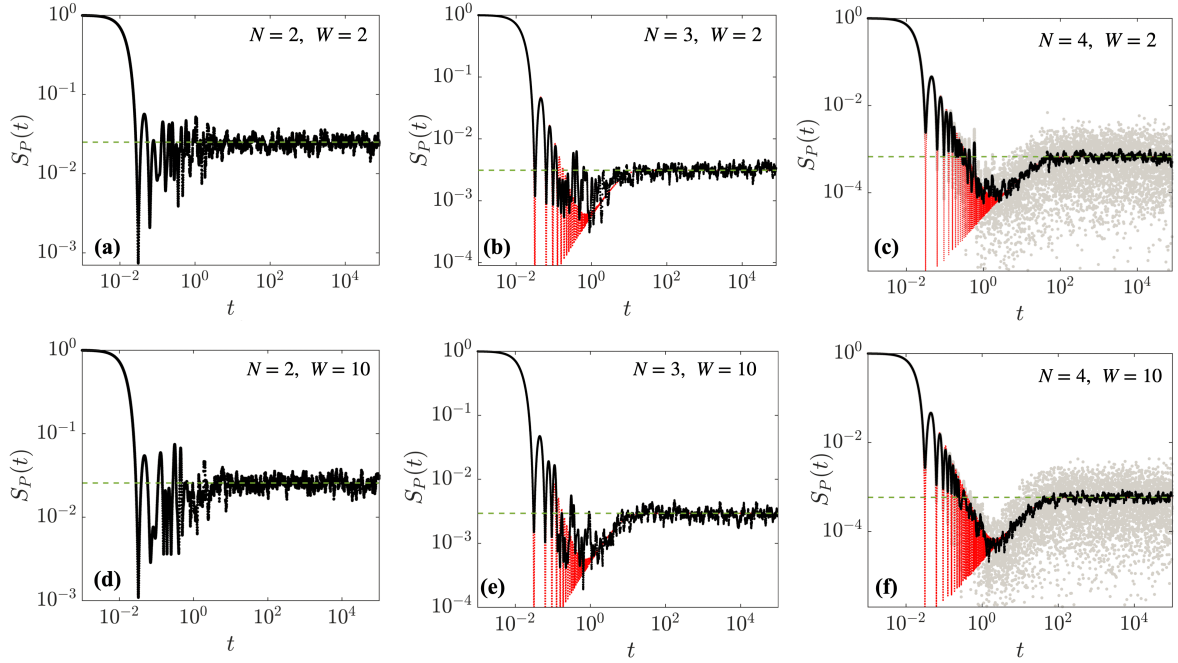
Figure 7: Survival probability of (a,d) 2 particles (b,e), 3 particles, and (c,f) 4 particles. The number of wells is (a-c) W = 2 and (d-f) W = 10 . The initial state is a square distribution centered at E_{\text{mid}} = 700 and of width \Delta E = 100 . Black lines are the moving time averages on the logarithmic timescale with window [\log_{10} t - \Delta t, \log_{10} t + \Delta t] and \Delta t = 0.02 . Green horizontal dashed line indicates the infinite time average of the survival probability S_{\infty} . For N = 3 and 4, red lines represent the analytic solution. For N = 4 , the grey points represent the unaveraged value for comparison. The parameters used for each row correspond to those that give the minimum kurtosis for 4 particles in Fig. 5, namely \gamma = 30 and \tau = 15 for W = 2 , and \gamma = 20 and \tau = 7.5 for W = 10 .
