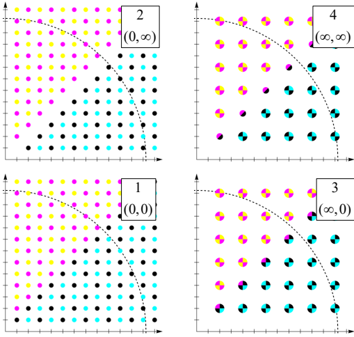
Figure 9: These four diagrams depict the spectrum for the four solvable cases of N = 2 particle and W = 2 wells; c.f. Fig. 1 and Sec. 3.1. Model 1: no interactions or barriers; model 2: infinite interactions no barriers; model 3 no interactions, infinite barriers; model 4 infinite interactions and barriers. Each dot represents an energy eigenstate with energy E = n_1^2 + n_2^2 given by the sum of the squares of the integer coordinates (n_1, n_2) of the point. States with n_1 \geq n_2 represent the symmetrized states with positive parity in black and with negative parity in cyan. States with n_1 < n_2 represented by magenta and yellow dots are antisymmetric and have negative and positive parity, respectively. In models 1 and 2, all states are two-fold degenerate except in model 1 (no barriers, no interactions) when n_1 = n_2 . Additionally, models 3 and 4 have additional two-fold degeneracies (in model 4, states along the diagonal represented by split dots with twice the area), four-fold (in model 4, represented by quartered dots along the diagonal) and eight-fold (in models 3 and 4, represented by pairs of quartered dots with exchanged integer quantum numbers). The dashed quarter-circle is the boundary E = 150 with radius \sqrt{150} and is included to aid visualization of the spectral flow.
