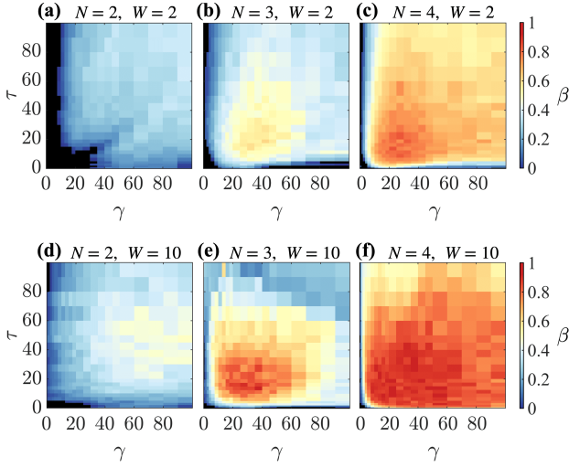
Figure 4: Brody distribution parameter \beta as a function of \tau and \gamma for (a,d) N = 2 , (b,e) N = 3 , and (c,f) N = 4 particles. The number of wells are (a-c) W = 2 and (d-f) W = 10 . For W = 2 wells the maximum \beta_{max} = 0.8269 is found for N = 4 particles at \gamma = 20 and \tau = 12.5 , while for W = 10 , we find \beta_{max} = 0.9512 for N = 4 particles at \gamma = 45 and \tau = 12.5 . Black areas show \beta < 0 indicating degeneracies and picket-fence spectra.
