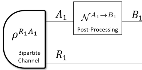
Figure 3: A state \rho^{R_1 A_1} represents a special type of bipartite channel, and a standard EBC can be seen as an EBSC post-processing map.
