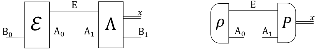
Figure 7: (Left) Implementation of a quantum super-instrument. A CPTP map \mathcal{E} is performed as pre-processing while a quantum instrument \Lambda = \sum_x \Lambda_x \otimes |x\rangle\langle x| encompasses the post-processing. (Right) A POVM of quantum channels. The pre-processing is a quantum state \rho and the post processing is a bipartite measurement channel P = \sum_x \text{Tr}_x(\cdot P_x) \otimes |x\rangle\langle x| for POVM \{P_x\}_x .
