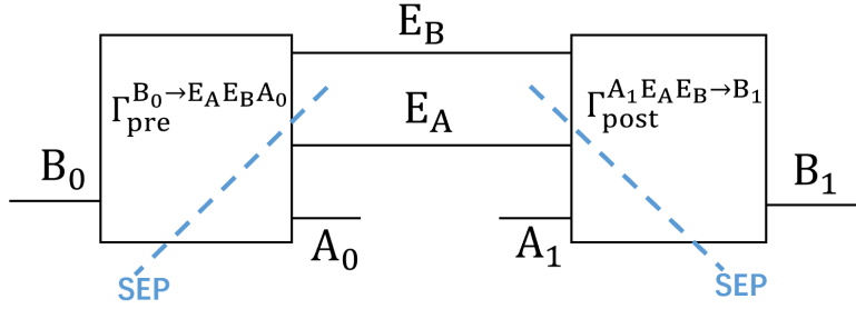
Figure 6: A general way to implement an EB supermap. \Gamma_{\text{pre}}^{B_0 \rightarrow E_A E_B A_0} is partly EB for the output system E_A A_0 and \Gamma_{\text{post}}^{A_1 E_A E_B \rightarrow B_1} is partly-EB for the input system E_A A_1 .
