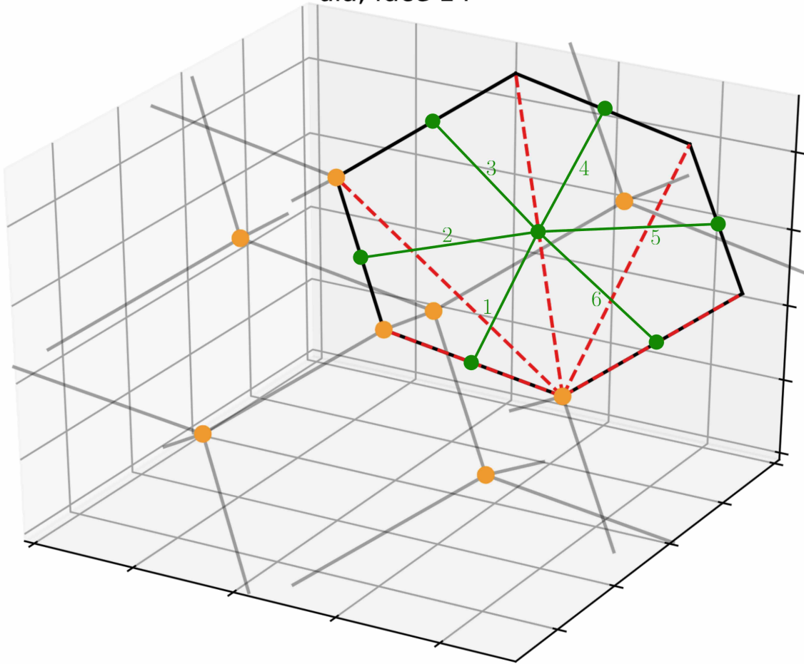
Figure 14: A guiding example for reading the gate orderings in lib/doc taken from the 14th face of the decoder graph of the diamond (dia) lattice. Here, the green is overlaid on the actual decoder graph shown in lib/doc . Qubits and CZ gates (green) are placed on edges and faces. The red dotted lines indicate correlated errors due to X -type errors. The gate ordering always begins with a CZ gate supported on a qubit causing a weight one error, and ends with a CZ gate supported on a qubit causing a weight one error. The ordering proceeds either clockwise or counter-clockwise (the choice of which, in our error model, will not have an effect); in this case, it is labeled clockwise. The unit cell vertices and edges of the tiling are depicted in yellow and black and grey, respectively.
