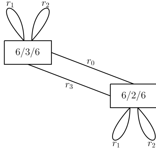
The duality isomorphism is the identity.
