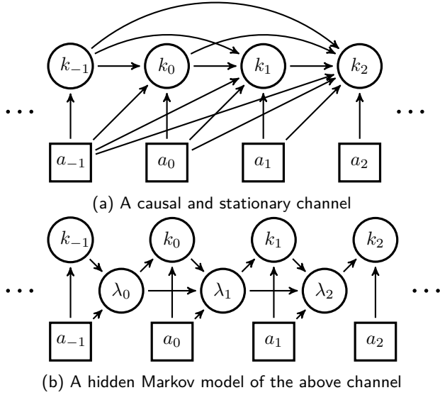
Figure 3: Influence diagrams [60] for stochastic channels. The boxes represent choices made by the experimenter, circles represent random variables, and arrows represent a possible causal influence. Note that no arrows point backwards in time, and that in the hidden Markov model the state \lambda_t mediates all causal influences through time.
