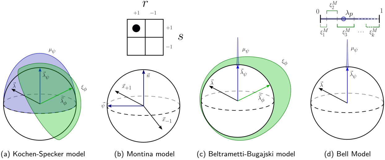
Figure 1: Visualizations of the state space, preparation distributions, and response functions for (a) the Kochen-Specker model, (b) Montina's model, (c) the Beltrametti-Bugajski model for d = 2 , and (d) Bell's model for d = 2 . Blue represents the support of preparations, and green the support of the response functions, where possible. Black objects are generic elements of the state space.
