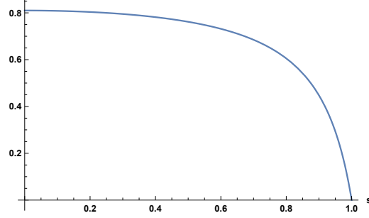
Figure 1: The SDPI constant \eta_{\chi_\kappa^2}(\mathcal{E}, \sigma) with respect to s , for BSC(0.05).
