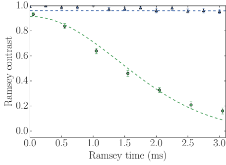
Figure 5: Coherence decay of the qubit in encoding A without (blue triangles) and with (green circles) additional magnetic field noise.
