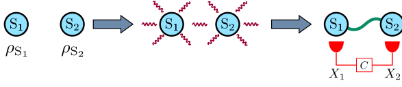
Figure 2: Schematic illustration of the measurement of the lower bound of \bar{I} . The system is prepared in a separable state \rho = \rho_{S_1} \otimes \rho_{S_2} and correlations of the observables X_1 and X_2 are measured after the evolution.
