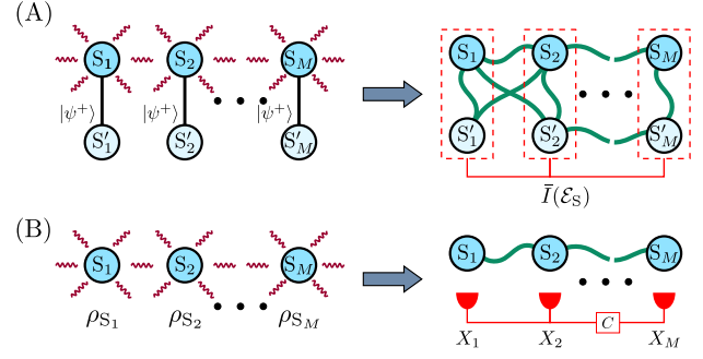
Figure 3: Schematic illustration of the multipartite correlation measure. (A) Choi-Jamiołkowski representation of the dynamics. The system is prepared in a product of maximally entangled states of 2M parties \{S_j|S'_j\} and the dynamics affect only the subsystems S_j . If and only if the dynamics are correlated, the bipartitions \{S_j S'_i | S_j S'_j\} will be entangled, yielding a nonzero \bar{I} . (B) Schematic depiction of the procedure to estimate a lower bound of \bar{I} . There, the system is prepared in a separable state \rho_{S_1} \otimes \rho_{S_2} \cdots \otimes \rho_{S_M} and correlations in the dynamics appear as correlations C (see page 4) in a measurement of the observables X_j .
