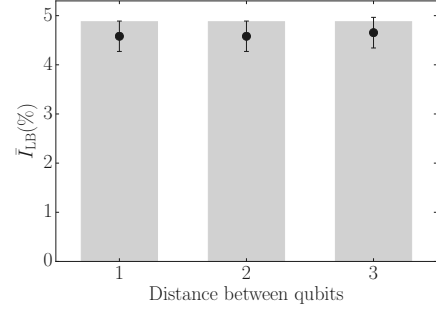
Figure 7: Lower bound for pairwise spatial correlations in a four-qubit system as a function of the distance (in terms of ion index difference in the ion string) to qubit 1, depicted with black circles. The corresponding simulations are shown with shaded bars. As all qubits have the same encoding, the correlations between qubit 1 and qubit 2, 3 and 4 respectively are the same within error bars.
