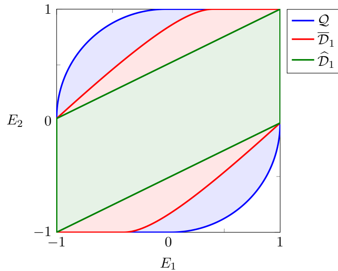
Figure 8: Comparison of the sets \bar{\mathcal{D}}_1 and \hat{\mathcal{D}}_1 , corresponding respectively to the max-average and max-peak assumptions, for \omega_1 = \omega_2 = 0.15 , illustrating that the latter of the two assumptions puts a stronger constraint on the behavior of the devices. The quantum set \mathcal{Q} is also represented for comparison.
