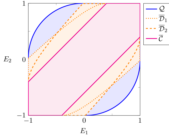
Figure 7: Representations of the sets \bar{\mathcal{C}} , \bar{\mathcal{D}}_1 , \bar{\mathcal{D}}_2 , and \mathcal{Q} for \omega_1 = \omega_2 = 0.15 . Since the quantum region is strictly larger than the individual sets \bar{\mathcal{D}}_x (or even than their convex combination), it is possible to certify the production of genuine randomness.
